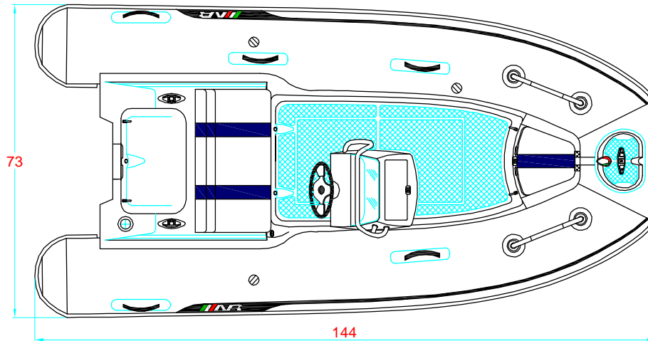
PLANT VIEW VISTA SUPERIOR
